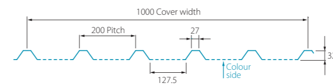
RL32 liner, trough perforated
