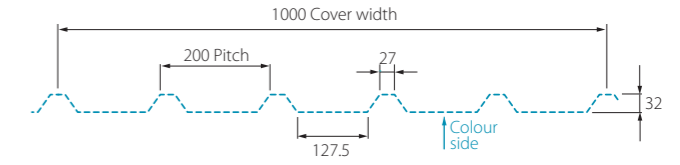
RL32 liner, fully perforated
