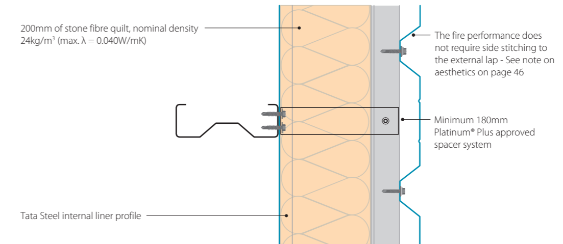
Vertical sections
